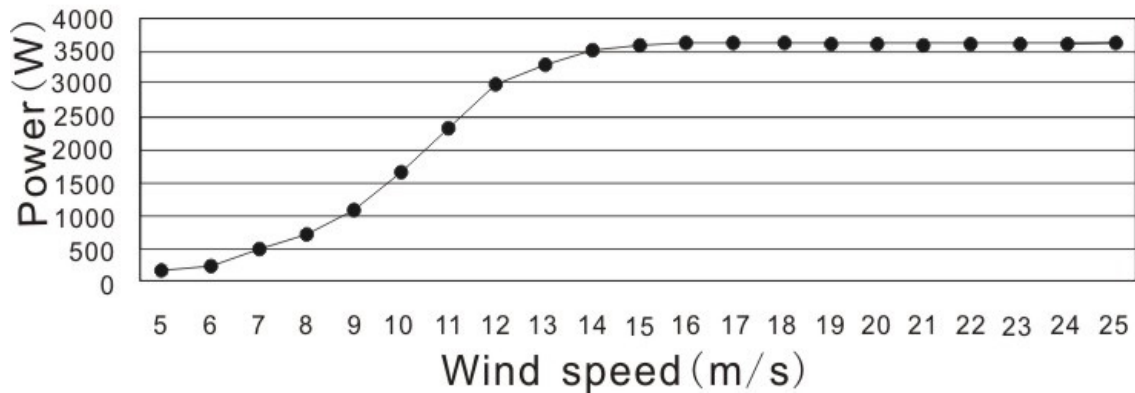
Wind velocity/Power Curve
