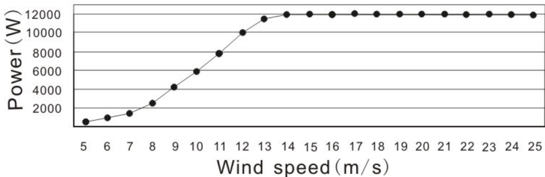
Wind velocity/Power Curve
