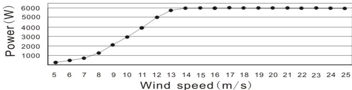
Wind velocity/Power Curve
