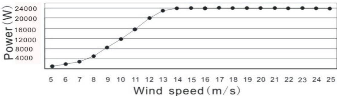
Wind velocity/Power Curve
